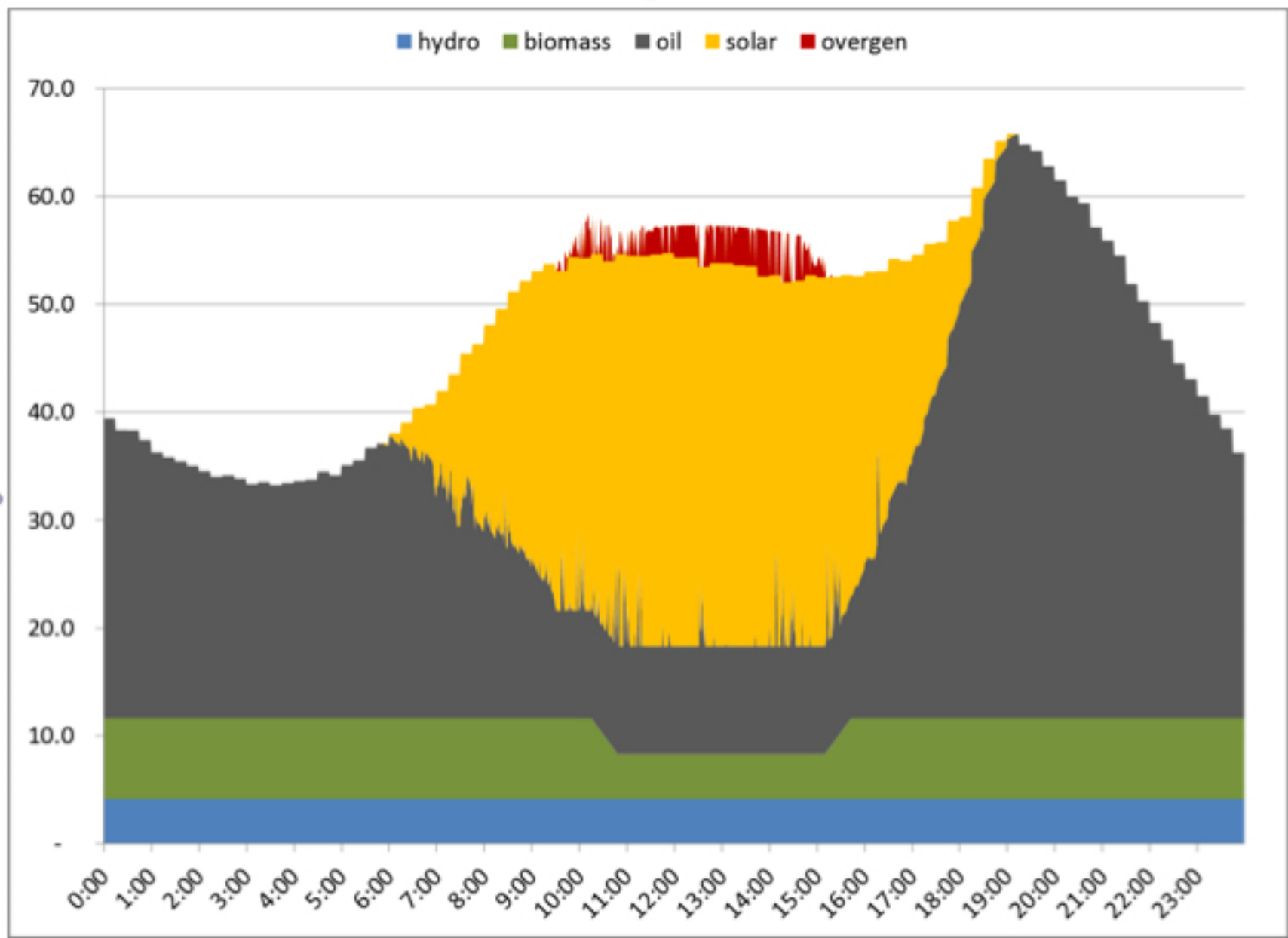
Figure 2 - 2015 Worst-case solar day (showing over generation in red)
